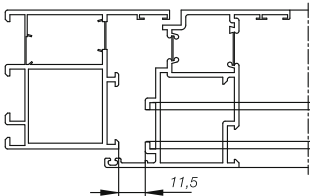
Vertical section KSP on the aluminium window
