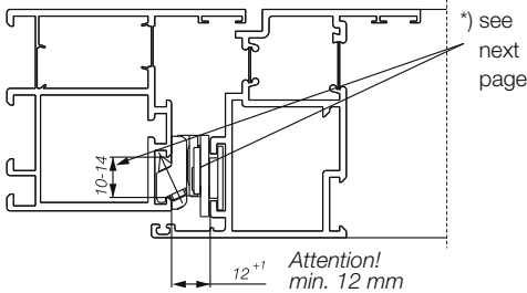
Vertical section KSP on the aluminium window
