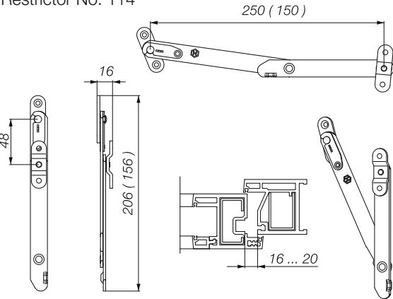
Restrictor No. 114
