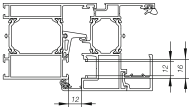
Vertical section KSP on the timber window
