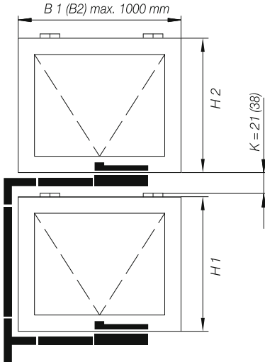
PRIMAT-A, type: f, 2 sashes, on top of each other Space requirements between the sashes measured from the bottom edge of the upper sash to the hinges of the lower sash (measure K): 21 mm with stay holder 1 38 mm with stay holder 2
