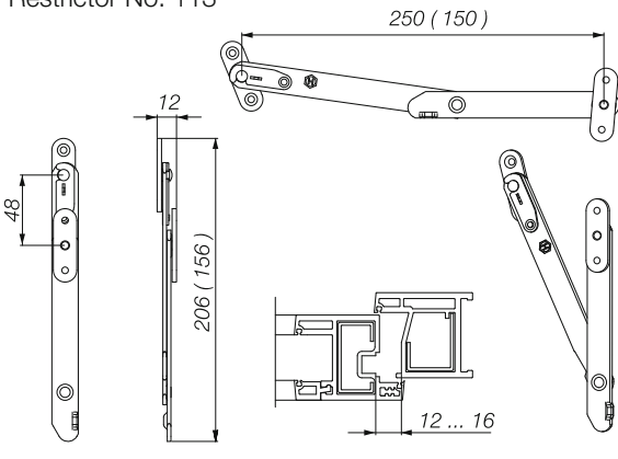
Restrictor No. 113
