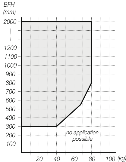
Application diagram for restrictors, application in pairs.
