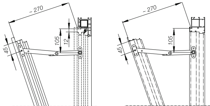
Restrictor on PVC and aluminium windows
