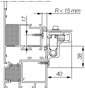
Vertical section on the Alu window with stay holder 2
